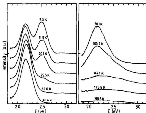
FIG. 4. Luminescence of uncolored \text{CdI}_2:\text{CuI} (5 mole% of \text{CuI} ).
