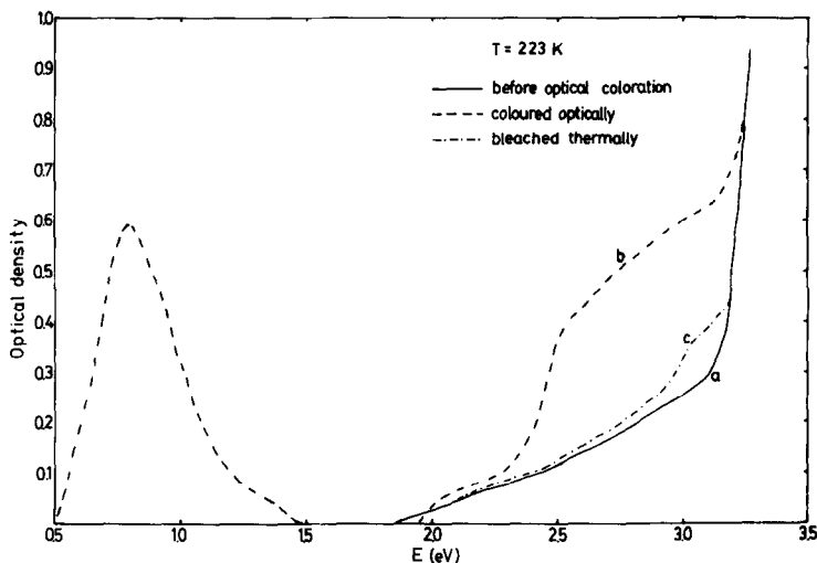
FIG. 2. Absorption spectrum of \text{CdI}_2:\text{CuI} (1 mole% of CuI) at 223 K. The crystal had a thickness of 1250\ \mu\text{m} .
