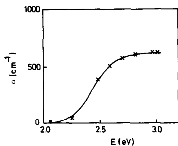
FIG. 7. Absorption coefficient \alpha of Cu aggregates in \text{CdI}_2 .
