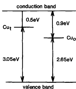
FIG. 5. Energy level diagram of Cu atoms in tetrahedral ( \text{Cu}_t ) and octahedral ( \text{Cu}_o ) sites in \text{CdI}_2 .
