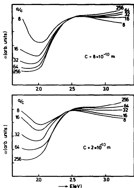
FIG. 6. Calculated absorption coefficients \alpha of \text{CdI}_2 containing ellipsoidal Cu particles. In each plot the c axis of the ellipsoid is constant. The numbers for the different curves give the ratio m = a/c . The curves are scaled to one another with the volume fraction F .
