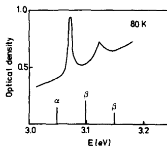
FIG. 1. Absorption spectrum of \text{CdI}_2:\text{CuI} (3 mole% of \text{CuI} ) at 80 K. The spectral resolution is 0.005 eV. The crystal had a thickness of 400 \mu\text{m} . The lines in the lower part give the position of exciton peaks in \alpha - \text{CuI} and \beta - \text{CuI} .
