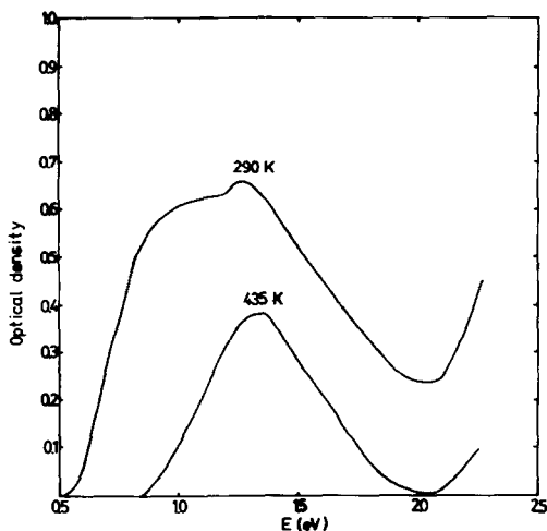
FIG. 3. Absorption spectrum of \text{CdI}_2:\text{CuI} (1 mole% of CuI) at 290 and 435 K, after many optical coloration–thermal bleaching cycles.
