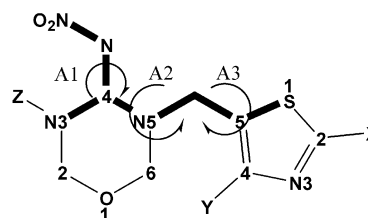
Figure 2. Structures and dihedral angles of thiamethoxam and hapten candidates.
