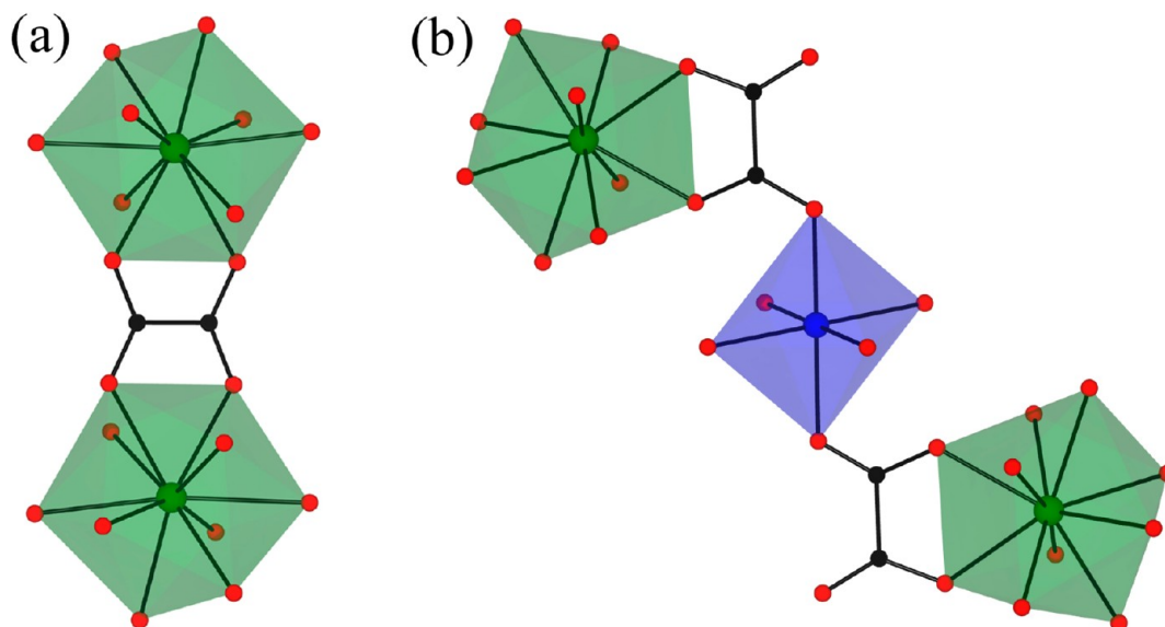
Figure 5. Connectivity between the U^{4+} cation and M^{2+} ( M = Mn^{2+} , Fe^{2+} , Co^{2+} , and Zn^{2+} ) cations. All four oxygen atoms in the oxalate ligand are bonded to two U^{4+} cations in part a, whereas in part b three oxygen atoms in the oxalate ligand are linked to the U^{4+} and M^{2+} cations leaving one oxygen atom in a terminal position. For the sake of clarity, the H atoms around the M^{2+} cation are omitted.
