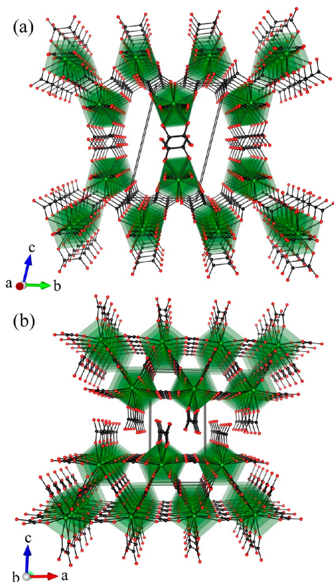
Figure 3. Polyhedral diagram of layers composed of the \text{U}^{4+} cations and oxalate anions for \text{Na}_2\text{U}_2\text{M}(\text{C}_2\text{O}_4)_6(\text{H}_2\text{O})_4 ( \text{M} = \text{Mn}^{2+} , \text{Fe}^{2+} , \text{Co}^{2+} , and \text{Zn}^{2+} ) along the (a) a - and (b) b -axis are shown. For clarity, the \text{M}^{2+} cations and water molecules are omitted.
