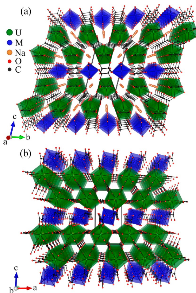
Figure 2. Polyhedral structure representation of \text{Na}_2\text{U}_2\text{M}(\text{C}_2\text{O}_4)_6(\text{H}_2\text{O})_4 ( \text{M} = \text{Mn}^{2+} , \text{Fe}^{2+} , \text{Co}^{2+} , and \text{Zn}^{2+} ) along the (a) a - and (b) b -axis. The three-dimensional network consists of \text{UO}_{10} and \text{MO}_6 polyhedra bridged by oxalate groups. For clarity, the H atoms of water molecules attached to the \text{M}^{2+} cations are omitted.
