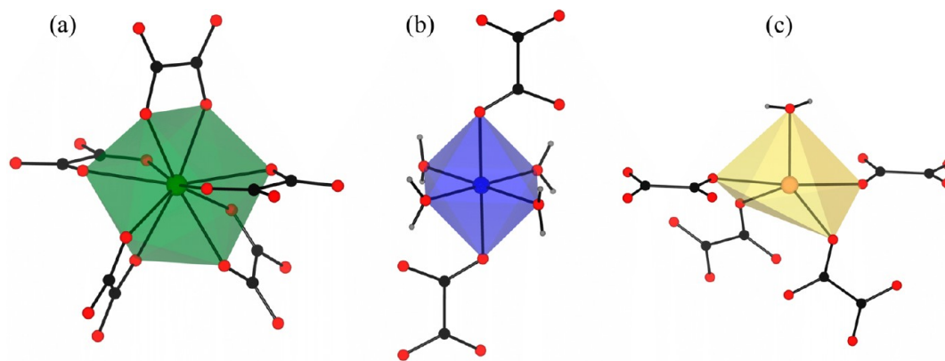
Figure 4. Local coordination environments of \text{Na}_2\text{U}_2\text{M}(\text{C}_2\text{O}_4)_6(\text{H}_2\text{O})_4 ( \text{M} = \text{Mn}^{2+} , \text{Fe}^{2+} , \text{Co}^{2+} , and \text{Zn}^{2+} ). The \text{U}^{4+} cation is surrounded by five oxalate ligands (a), the \text{M}^{2+} cations are bonded to four water molecules and two oxalate groups (b), and the \text{Na}^+ cation is linked to one water molecule and four oxalate groups (c).
