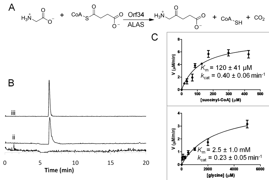
Figure 2. Characterization of ORF34 as a 5-aminolevulinate synthase. (A) Schematic of the condensation of glycine and succinyl-CoA to yield 5-aminolevulinic acid catalyzed by ORF34. (B) Extracted ion chromatograms ( m/z = 132 [M + H]^+ ) showing ORF34-catalyzed production of ALA (trace ii) as compared to the ALA standard (trace iii). ALA was not detected in controls without ORF34 (shown, trace i) or without any of the substrates (not shown). (C) Determination of ORF34 kinetic parameters by assay with DTNB. Parameters were determined for succinyl-CoA (top panel) by fixing the glycine concentration at 10 mM, while parameters were determined for glycine (bottom panel) by fixing the succinyl-CoA concentration at 500 \mu\text{M} . Error bars represent standard deviations from at least three independently performed experiments.
