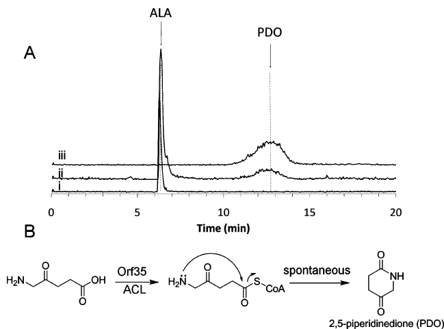
Figure 4. Instability of ALA-CoA. (A) Extracted ion chromatograms ( m/z = 114 [ M + H ] ^+ ) showing the formation of PDO in the reaction mixture of ORF35 (trace ii). PDO standard is shown in trace iii and the no enzyme control is shown in trace i. (B) Schematic of the spontaneous cyclization of ALA-CoA to PDO.
