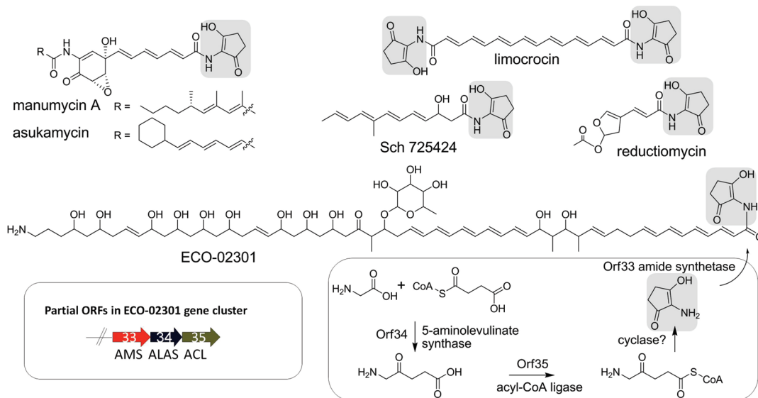
Figure 1. Examples of natural products containing C_5N (shaded). Candidate ORFs and a putative biosynthetic pathway for C_5N formation during ECO-02301 biosynthesis are boxed. ALAS, 5-aminolevulinic synthase; ACL, acyl-CoA ligase; AMS, amide synthetase.
