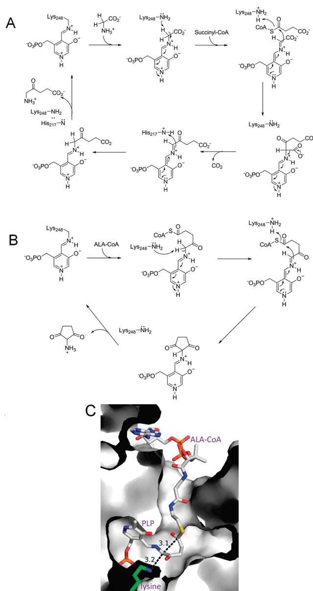
Figure 8. Proposed PLP-dependent catalytic mechanism of ORF34. (A) Mechanism for ALA synthesis. In the substrate-free state, PLP is bound by enzyme (internal aldimine). The incoming glycine induces transaldimination, leading to the PLP-Gly adduct (external aldimine). The electrophilic substrate succinyl-CoA is attacked by the PLP-activated glycine, leading to C-C bond formation with the release of CoASH. Decarboxylation and reprotonation result in formation of the PLP-ALA adduct that is finally released to regenerate the internal aldimine. (B) Mechanism for C 5 N synthesis. ALA-CoA induces transaldimination, yielding the ALA-CoA-PLP complex. The thioester carbonyl in ALA-CoA is then attacked by the PLP-activated ALA moiety intramolecularly, leading to C-C bond formation with the release of CoASH. The PLP-C 5 N complex is finally released to regenerate internal aldimine. (C) Three-dimensional structural model of the ORF34 active site. The structure was modeled on the Rhodobacter capsulatus ALAS using the online program HHPred, and the substrates were docked using the software GOLD.
