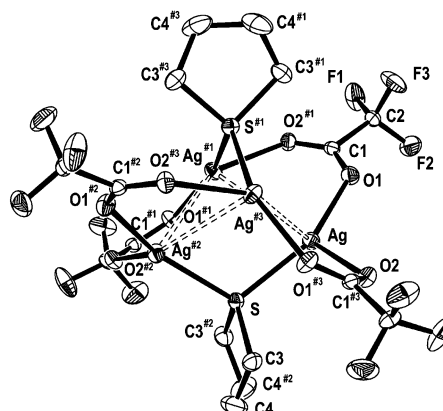
Figure 1. Molecular structure of complex 1 with the labeling scheme of the atom positions. Hydrogen atoms have been omitted for clarity.
