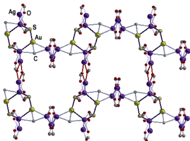
Figure 4. Polymeric layer structure of complex 3 . Hydrogen and fluorine atoms, as well as the carbon atoms of the tht and mes ligands (except the ipso carbon), have been omitted for clarity reasons. Hexanuclear \text{Ag}_2\text{Au}_2\text{S}_2 rings are marked in black and Ag–O–Ag bridges in red.
