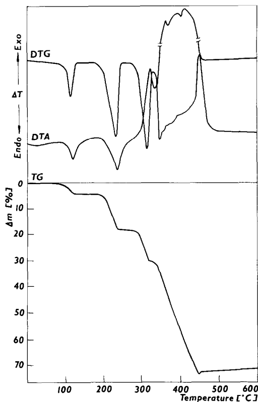
Fig. 2. TG, DTG and DTA curves of \text{Ni(en)}_3\text{Ni(CN)}_4 \cdot \text{H}_2\text{O} (pH 12).
