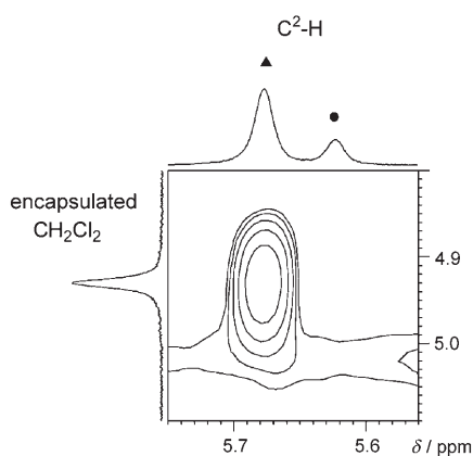
Figure 6. Section of the ^1\text{H}, ^1\text{H} ROESY spectrum of a solution of 1a-1a in \text{CDCl}_3 ( 1.1 \times 10^{-2} \text{ M} ) in the presence of a 30-fold excess of \text{CH}_2\text{Cl}_2 , at 223 K. The cross peak relating the resonances assigned to the encapsulated \text{CH}_2\text{Cl}_2 and the \text{C}^2\text{-H} protons of 1a-1a-CH 2 Cl 2 (marked with a triangle) is shown. The resonance of the \text{C}^2\text{-H} protons of 1a-1a-CDCl 3 is marked with a circle. The plotting cut-off levels are the same as those in Figure 5.
