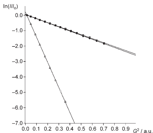
Figure 7. Plot of \ln(I/I_0) versus arbitrary units proportional to the square of the gradient amplitude, for a ^1\text{H} PGSE diffusion measurement of a 2 \times 10^{-3} \text{ M} solution of 1a·1a in \text{CDCl}_3 plus a 20-fold excess of \text{CH}_3\text{I} . The measurements on the resonances of the capsule in 1a·1a · \text{CDCl}_3 (○) and 1a·1a · \text{CH}_3\text{I} (●), as well as on the resonance from the encapsulated \text{CH}_3\text{I} (□) afford very similar intensity decays, while on the resonance from the free \text{CH}_3\text{I} (△) the intensity decay is much stronger, indicating a much larger D value. Diffusion parameters (see the Experimental Section): \Delta = 65.5 \text{ ms} , \delta = 4.5 \text{ ms} , number of scans = 40.
