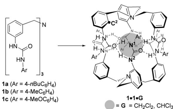
Scheme 1. Tris(3-ureidobenzyl)amines 1a–c (left) dimerise in non-competitive solvents to form molecular capsules in which guests can be accommodated (right).
