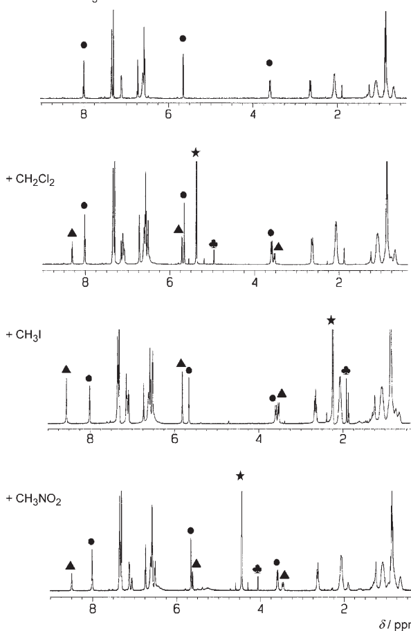
Figure 1. Sections of the 1 H NMR spectra at 213 K for solutions of 1a•1a in CDCl 3 (2 × 10 −3 M) before and after addition of a 20-fold excess of guest (CH 2 Cl 2 , CH 3 I and CH 3 NO 2 ). Selected peaks from 1a•1a •CDCl 3 (N 1 –H, C 2 –H and one amine methylenic proton, see Scheme 1, and Figure S1 in the Supporting Information) are marked with circles, [10] the corresponding resonances from 1a•1a • G are indicated with triangles, the guest within 1a•1a is distinguished by a trefoil and the free guest with a star. The resonances from chloroform are overlapped with those of the capsule. The spectra are truncated in the upper part.
