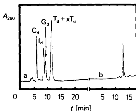
Fig. 10. HPLC profile after enzymatic tandem hydrolysis of d(G-T-A-G-A-xT-xT-C-T-A-C)_2 ( 9 ; 1.2 \mu M of double strand) with calf-spleen phosphodiesterase and alkaline phosphatase after a total incubation time of 70 h at 37°. Trace a, solvent system III; trace b, solvent system II, following solvent system III. Conditions, see Exper. Part .
