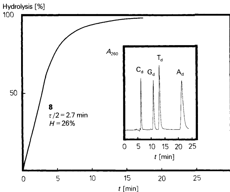
Fig. 8. Time course of phosphodiester hydrolysis of d(G-T-A-G-A-A-T-T-C-T-A-C)_2 ( 8 ) with calf-spleen phosphodiesterase and alkaline phosphatase (23°; conditions, see Exper. Part ; 1.2 \mu M of double strand) and HPLC profile (insert) after enzymatic tandem hydrolysis of 8 with calf-spleen phosphodiesterase followed by alkaline phosphatase (conditions, see Exper. Part ).
