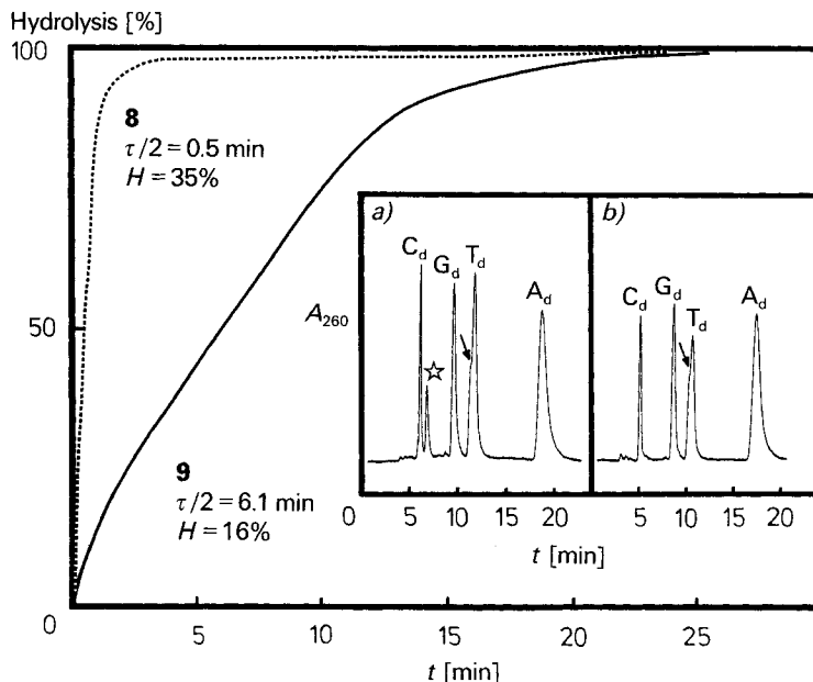
Fig. 7. Time course of phosphodiester hydrolysis of d(G-T-A-G-A-xT-xT-C-T-A-C)_2 ( 9 ; —), and d(G-T-A-G-A-T-T-C-T-A-C)_2 ( 8 ; ----) with snake-venom phosphodiesterase and alkaline phosphatase (23°; conditions, see Exper. Part; 1.2 \mu M of each double strand) and HPLC profiles (insert) after enzymatic tandem hydrolysis of 9 with snake-venom phosphodiesterase followed by alkaline phosphatase, a) after a total incubation of 75 min (37°) and b) after additional incubation for 30 min at 37° (conditions, see Exper. Part). ☆: xT_d 5'-monophosphate ( pxT_d ); \rightarrow : xT_d .
