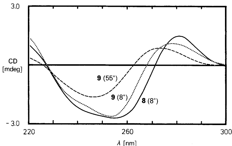
Fig. 5. CD Spectra of d(G-T-A-G-A-xT-xT-C-T-A-C)_2 ( 9 ; ·····) and d(G-T-A-G-A-A-T-T-C-T-A-C)_2 ( 8 ; —) at 8° and of 9 at 55°. Oligomer conc., 1.2 \mu M of double strand; buffer, see Fig. 1.
