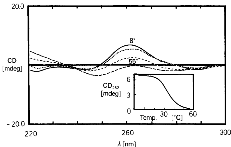
Fig. 4. CD Spectra of d(A_{12}) \cdot d[(xT)_{12}-T] ( 7 \cdot 5 ; 2 \mu\text{M} single-strand conc.) at temperatures between 8 and 55^\circ . Buffer, see Fig. 1. Insert: ellipticity at 262 nm as a function of temp.
