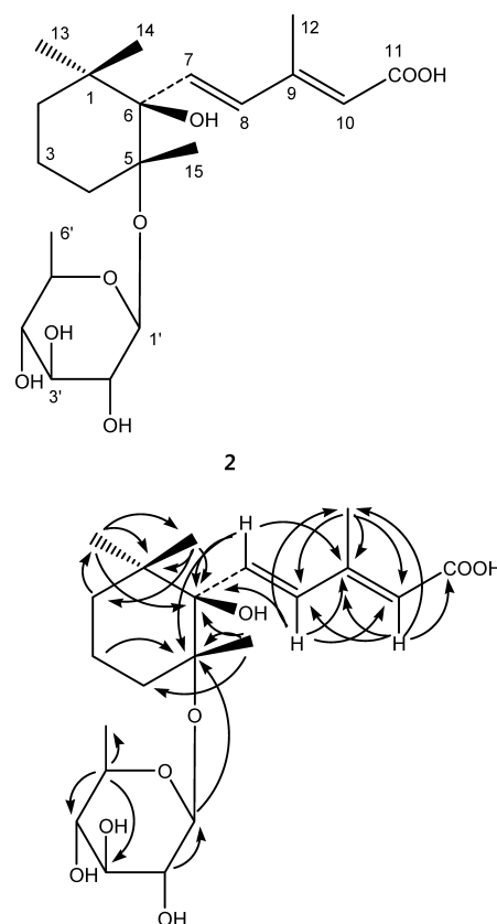
Fig. 2. Key HMBC Correlations for 2
