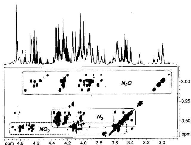
Fig. 5. Section of the ^1\text{H} TOCSY spectrum for [\text{Mo}_3\text{S}_4(\text{taci})_3]^{4+} ( \text{D}_2\text{O} , pH 8, r.t., 11.4 Tesla, 150 ms MLEV-17 mixing with \gamma/2\pi B_1 \approx 8.6 KHz) with the conventional ^1\text{H} NMR spectrum plotted above. The three major coordination types are indicated.
