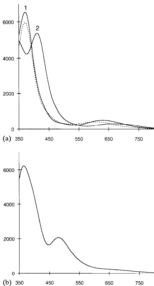
Fig. 2. (a) Vis spectrum of [\text{Mo}_3\text{S}_4(\text{taci})_3]\text{Br}_4 (1), [\text{Mo}_3\text{S}_4(\text{tdc})_3]\text{Br}_4 (2) and [\text{Mo}_3\text{S}_4(\text{H}_2\text{O})_9]^{4+} (dotted line). (b) Vis spectrum of [\text{Mo}_3\text{S}_4(\text{tdc})_3\text{CuBr}] .
