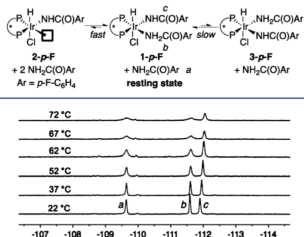
Figure 3. VT 19 F NMR spectroscopy of complex 1-p-F (resonances b and c ) with 1 equiv of 4-F-benzamide (resonance a ) in toluene.
