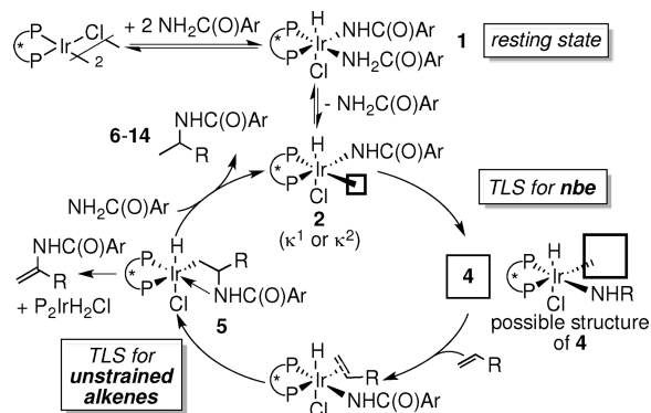
Scheme 2. Proposed Catalytic Cycle for the Ir-Catalyzed N–H Bond Addition of Arylamides to \alpha -Olefins
