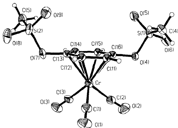
Fig. 1. Drawing of crystalline 2 including the labeling scheme. Hydrogen atoms have been drawn with arbitrarily small thermal coefficients for clarity. Selected bond distances (Å) Cr–C(11), 2.204(2); Cr–C(1), 1.874(8); S(1)–C(4), 1.722(8), S(1)–O(4), 1.617(5); S(1)–O(5), 1.409(7); C(11)–C(16), 1.398(1); C(11)–C(12), 1.439(1); C(12)–C(13), 1.378(1); C(13)–C(14), 1.415(1); C(14)–C(15), 1.420(1), C(15)–C(16), 1.393(1).
