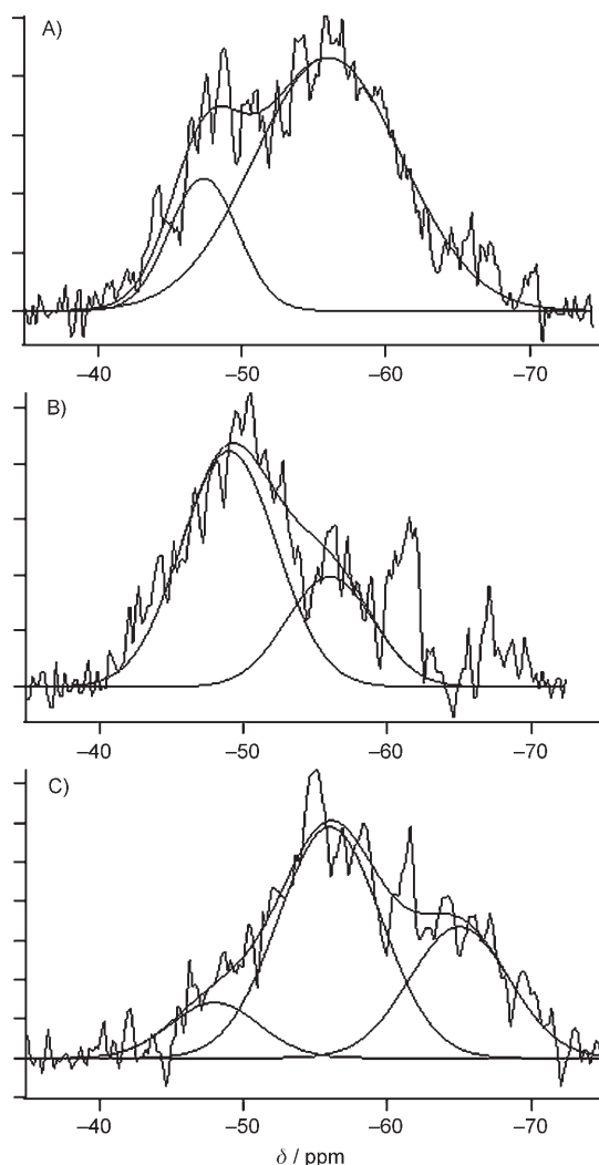
Figure 6. Solid-state ^{29}\text{Si} MAS NMR spectra of T^m sites. A) SA- \text{NEt}_2 , B) SA treated with a solution of DAPS in toluene for 5 min at room temperature (SA+DAPS), and C) SA-octyl.
