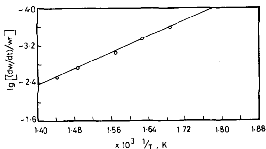
Fig. 3. Freeman-Carroll plot of cobalt chelate.
