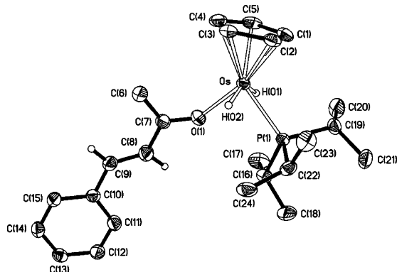
Figure 1. Molecular diagram of the cation of [OsH 2 (η 5 -C 5 H 5 ){κ 1 -OC(CH 3 )CH=CHPh}(P i Pr 3 )]BAr F 4 ( 3 ).
