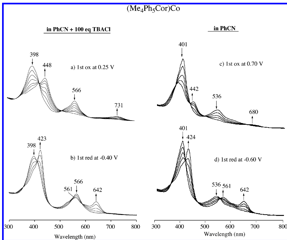
Figure 4. UV-visible spectral changes for (a) oxidation and (b) reduction of (\text{Me}_4\text{Ph}_5\text{Cor})\text{Co} in PhCN and 0.1 M TBAP containing 100 equiv of TBACl as compared to (c) oxidation and (d) reduction of the same solution not containing TBACl.
