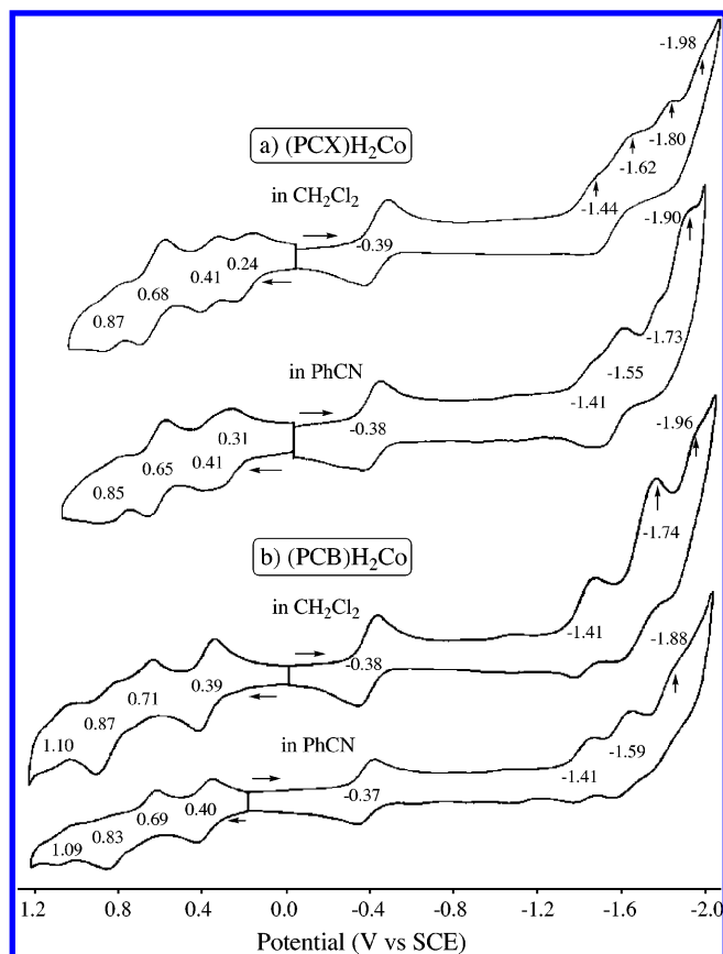
Figure 1. Cyclic voltammograms of (a) (PCX) \text{H}_2\text{Co} and (b) (PCB) \text{H}_2\text{Co} in \text{CH}_2\text{Cl}_2 or PhCN containing 0.1 M TBAP.
