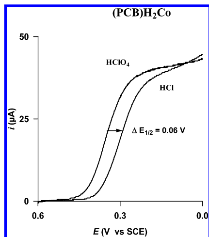
Figure 8. Reduction of O_2 at a rotating disk electrode coated with (PCB)- H_2Co in air-saturated 1 M HClO_4 or 1 M HCl . Rotating rate: 100 rpm. Scan rate: 5 mV/s.
