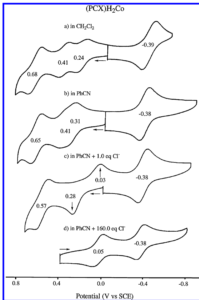
Figure 6. Cyclic voltammograms of (PCX) \text{H}_2\text{Co} in the following solutions containing 0.1 M TBAP: (a) \text{CH}_2\text{Cl}_2 , (b) PhCN, (c) PhCN + 1 equiv of TBACl, and (d) PhCN + 160 equiv of TBACl.
