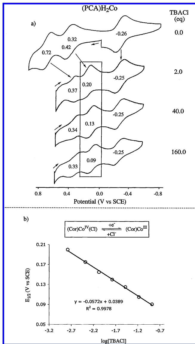
Figure 5. (a) Cyclic voltammograms of (PCA) \text{H}_2\text{Co} in PhCN and 0.1 M TBAP with added TBACl and (b) plot of E_{1/2} for the \text{Co}^{\text{IV}}\text{Cl}/\text{Co}^{\text{III}} process vs log [TBACl].
