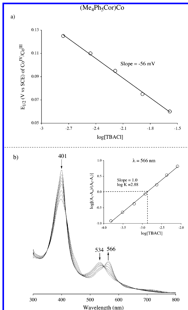
Figure 3. (a) Plot of E_{1/2} for the [\text{Co}^{\text{IV}}\text{Cl}_2]^-/[\text{Co}^{\text{III}}\text{Cl}]^- process of (\text{Me}_4\text{Ph}_5\text{Cor})\text{Co} in PhCN and 0.1 M TBAP vs \log [\text{TBACl}] added to solution and (b) UV–visible spectral changes of 2.5 \times 10^{-5} M (\text{Me}_4\text{Ph}_5\text{Cor})\text{Co} in PhCN with increasing TBACl concentrations from 1.5 \times 10^{-4} to 8.1 \times 10^{-3} M. Inset shows the Hill plot.
