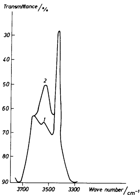
Fig. 6. Absorption spectra for calculation of the enol content in cyclohexanone
