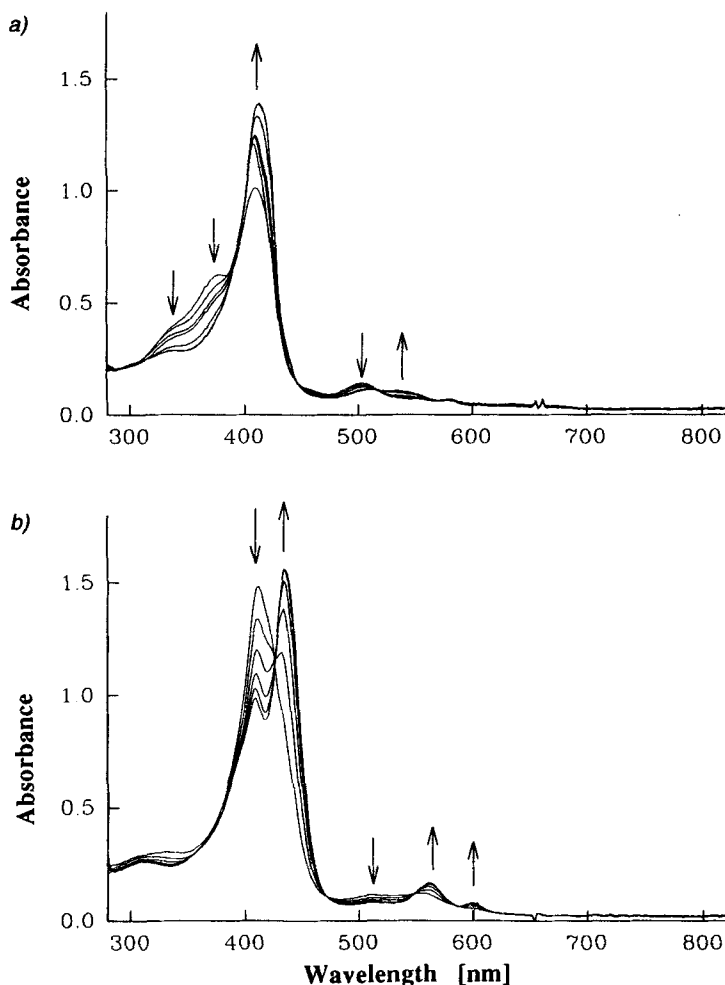
Fig. 7. Time-resolved UV/VIS spectroelectrochemistry on an OTTLE in \text{CH}_2\text{Cl}_2 (+ 0.1M \text{Bu}_4\text{NPF}_6 ) upon controlled-potential reduction of 4 \cdot \text{FeCl} at a) -0.9 \text{ V} vs. SCE (first reduction step) and b) at -1.6 \text{ V} vs. SCE (second reduction step)
