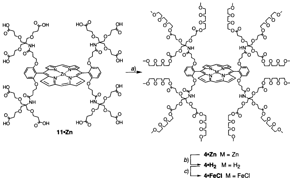
Scheme 3. Synthesis of the First Generation Dendritic Porphyrins 4·Zn , 4·H 2 , and 4·FeCl
