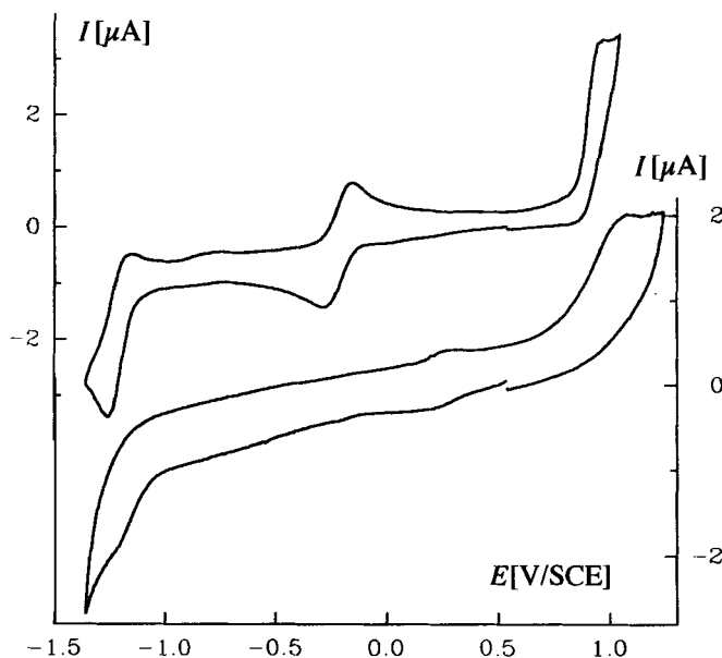
Fig. 8. Cyclic voltammograms of 4 \cdot \text{FeCl} (top) and 5 \cdot \text{FeCl} (bottom) in \text{H}_2\text{O} (+ 0.1M \text{Et}_4\text{NPF}_6 ) on a glassy carbon working electrode. Scan rate: 0.05 \text{ V s}^{-1} .
