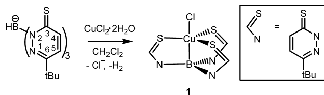
Scheme 1. Formation of Boratrane Compound [\text{Cu}\{\text{B}(\text{Pn}^{\text{tBu}})_3\}\text{Cl}] ( 1 ) and Numbering Scheme
