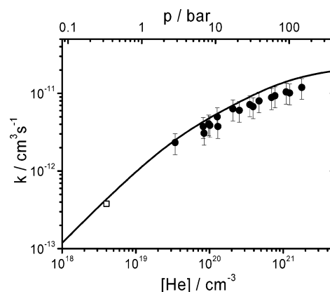
Figure 4. Falloff curve for helium at 600 K: ●, this work; □, ref 37; solid line, falloff curves calculated for R1 from eq 7; parameters for R1 are given in eq 14.
