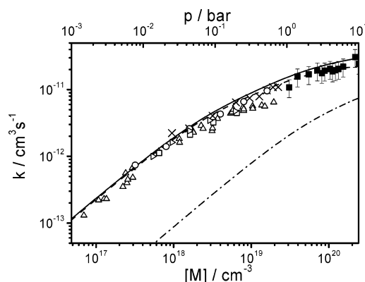
Figure 7. Falloff curve for nitrogen at 300 K: \circ : Ref. 37; open triangle facing right, ref 38; \triangle , ref 17; \square , ref 39; \times , ref 16; dashed and dashed dotted lines, falloff curves calculated from eq 7 for R1 and R2, respectively; solid line, sum of the two falloff curves. The falloff parameters for R1 and R2 are given in eq 16 and eq 17, respectively. In order to compare the literature data for N 2 with our results obtained in He, we scaled the gas density for the latter data by a factor of 0.64 ( k_{0,\text{He}}/k_{0,\text{N}_2} ) and added the results obtained in this way to the graph ( \blacksquare ).
