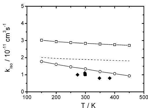
Figure 3. Calculated specific rate constants for the isotopic scrambling in the 18 OH + NO 2 reaction (open circles) compared to literature data (●, ref 19; ■, ref 7; ♦, ref 16). For comparison, k_{1,\infty} (open squares) and (2/3)k_{1,\infty} (dashed line) are added as well. See text for further explanations.
