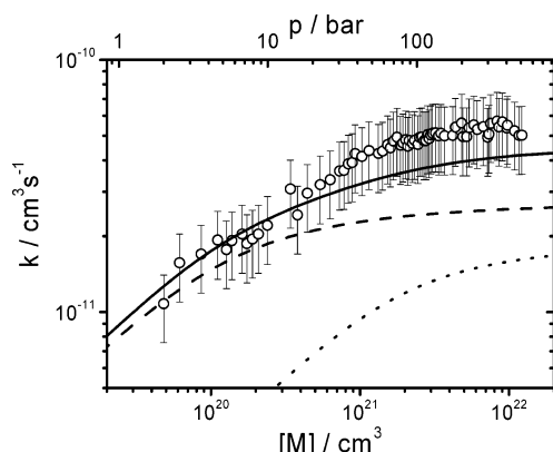
Figure 6. Falloff curve for helium at 300 K: \circ , k_1 + k_2 , this work; dashed and dotted lines, falloff curves calculated from eq 7 for R1 and R2, respectively; solid line, sum of the two falloff curves. The falloff parameters for R1 and R2 are given in eq 14 and eq 15, respectively.
