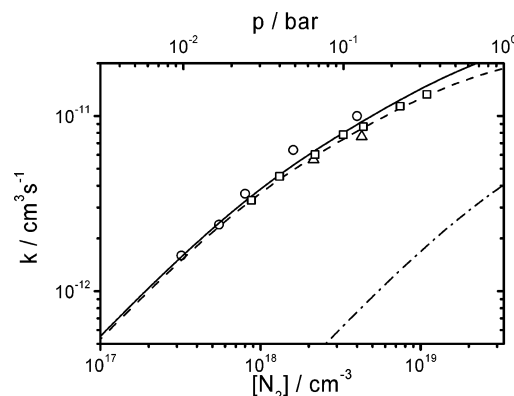
Figure 8. Falloff curve for nitrogen at 220 K: \circ , ref 37; \square , ref. 39; \triangle , ref. 40; dashed and dashed dotted lines, falloff curves calculated from eq 7 for R1 and R2, respectively; solid line, sum of the two falloff curves. The falloff parameters for R1 and R2 are given in eq 16 and eq 17, respectively.
