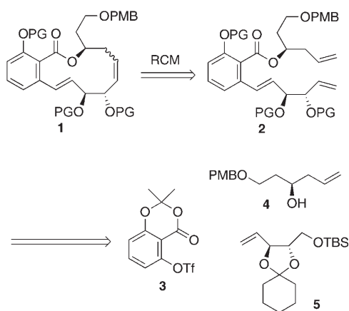
Scheme 1. Synthetic strategy for macrocycle 1 . PG: protecting group; PMB: para -methoxybenzyl; TBS: tert -butyldimethylsilyl; Tf: trifluoromethanesulfonyl.
