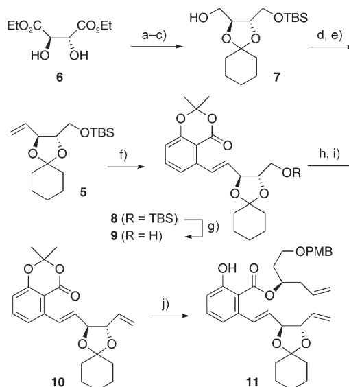
Scheme 2. Synthesis of the RCM substrate 11 from (+)-diethyl tartrate ( 6 ). a) Cyclohexanone, p -TsOH; b) LiAlH 4 ; c) NaH, TBSCl (73 %, 3 steps); d) SO 3 -Py, DMSO, Et 3 N (92 %); e) Ph 3 P=CH 2 , THF (76 %); f) 3 , Pd(OAc) 2 , Ph 3 P, Et 3 N, DMF (63 %); g) TBAF, THF (95 %); h) (COCl) 2 , DMSO, CH 2 Cl 2 ; then Et 3 N; i) CH 2 I 2 , Zn, Me 3 Al, THF (57 %, 2 steps); j) 4 , NaHMDS, THF (93 %). DMSO: dimethylsulfoxide; NaHMDS: sodium hexamethyldisilazide; p -TsOH: toluene-4-sulfonic acid; Py: pyridine; TBAF: tetrabutylammonium fluoride.
