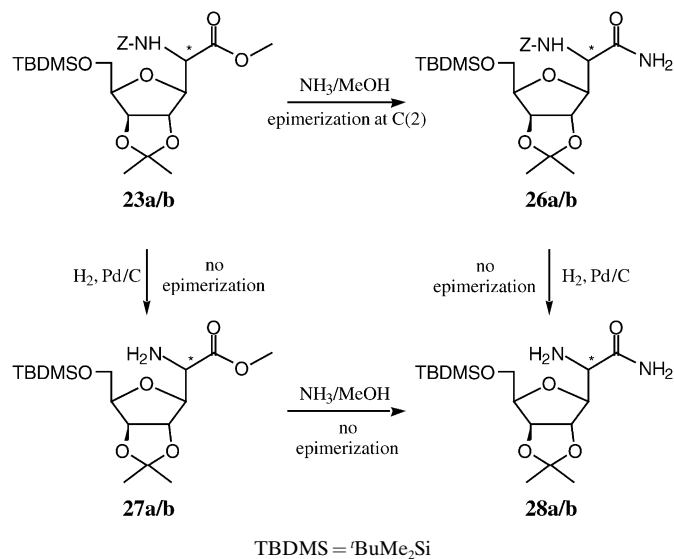
Scheme 11
