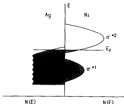
FIG. 3. Schematic density of states vs energy diagram showing splitting of the \sigma^* band and overlapping with 4d band of silver. ( \sigma^* results from the overlapping of Ni e_g -orbitals and O 2p -orbitals).
