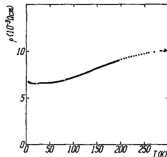
FIG. 1. Electrical resistivity of \text{AgNiO}_2 .
