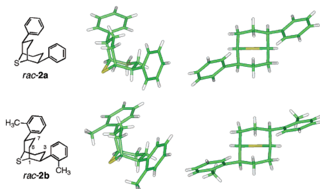
FIGURE 1. X-ray crystal structures of 2a and 2b . (Middle) View showing the chair/chair conformation of the bicyclic-nonane core. (Right) View down the \text{C}_2 symmetry axis. Relevant carbon position numbers are shown on the sketch of 2b .
