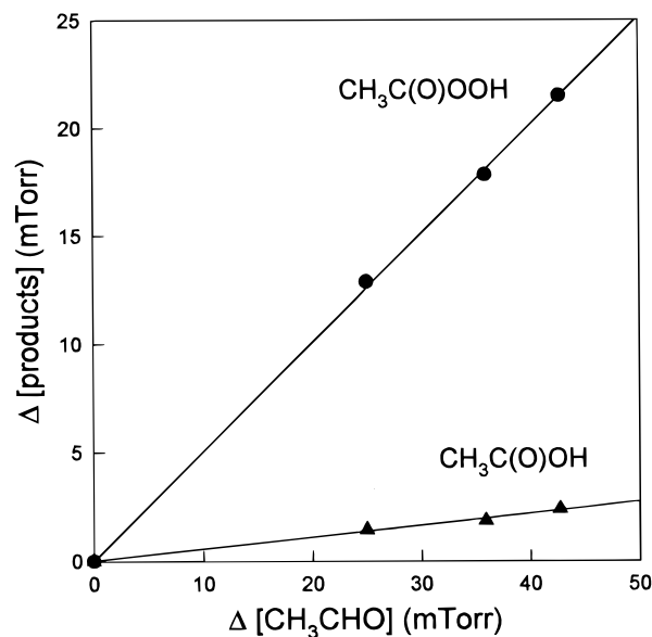
Figure 12. The formation of CH 3 C(O)OOH and CH 3 C(O)OH versus CH 3 CHO loss following UV irradiation of a mixture of 52.1 mTorr of CH 3 CHO, 26.1 mTorr of CH 3 OH, and 290 mTorr of Cl 2 in 700 Torr of air diluent.
