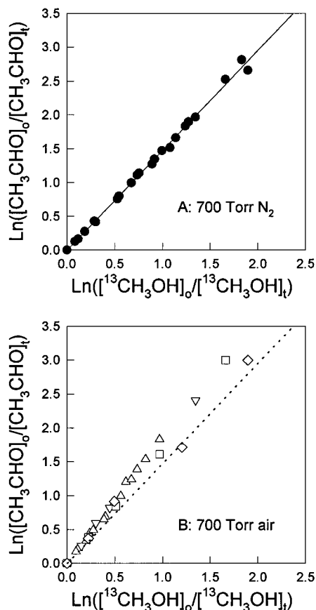
Figure 8. The loss of \text{CH}_3\text{CHO} versus ^{13}\text{CH}_3\text{OH} in 700 Torr of either (A) \text{N}_2 or (B) air diluent. Initial concentration ratios of [\text{CH}_3\text{OH}]_0/[\text{CH}_3\text{CHO}]_0 are 0.04–4.4 in the \text{N}_2 experiments and 0.04 ( \diamond ), 0.17 ( \square ), 1.7 ( \triangle ), and 2.4 ( \nabla ) for the experiments in air. The solid line in panel A is a linear least-squares fit of the data, which is reproduced as the dotted line in panel B.
