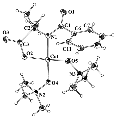
Fig. 1. ORTEP [29] plot of ( N -benzoyl-2-amino-2-methylpropanoato- O -)bis-(trimethylaminoxido)-copper(II).
