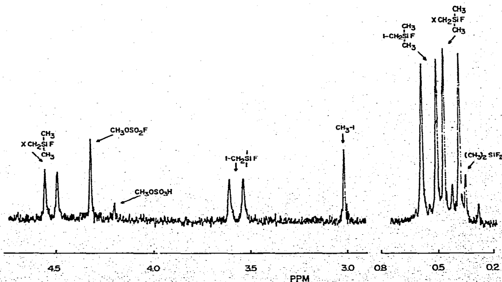
Fig. 2. The proton NMR of the reaction of (iodomethyl)dimethylfluorosilane with fluorosulfonic acid (X = OSO 2 F).
