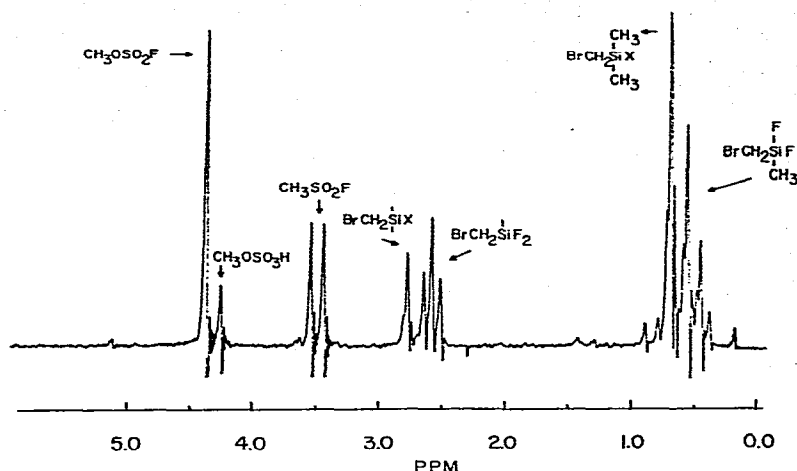
Fig. 1. The proton NMR of the reaction of (bromomethyl)dimethylsilyl fluorosulfonate with fluorosulfonic acid ( X = \text{OSO}_2\text{F} ).
