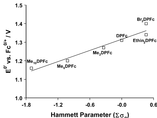
Figure 4. Linear relationship between E^0 and the Hammett substituent parameter for decaphenylferrocene and designated derivatives.
