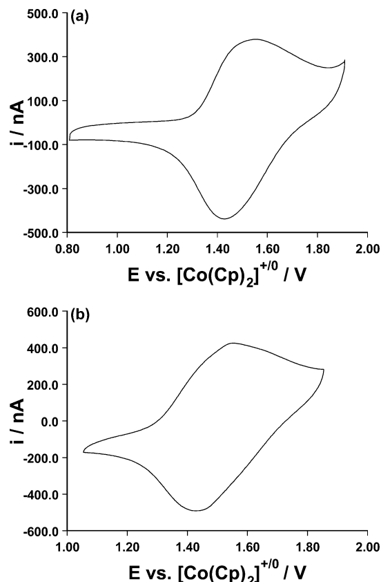
Figure 7. Cyclic voltammograms of (a) [DPFc + ][PF 6 − ] microparticles adhered to a 1 mm diameter GC electrode ( v = 0.1 \text{ V s}^{-1} ) in contact with bulk BMIM·PF 6 (scheme 2, Figure 1) and (b) as for (a) but with the microparticles being coated with a thin layer of BMIM·PF 6 prior to being placed in contact with aqueous (0.1 M KPF 6 ) electrolyte solution (scheme 3, Figure 1).
