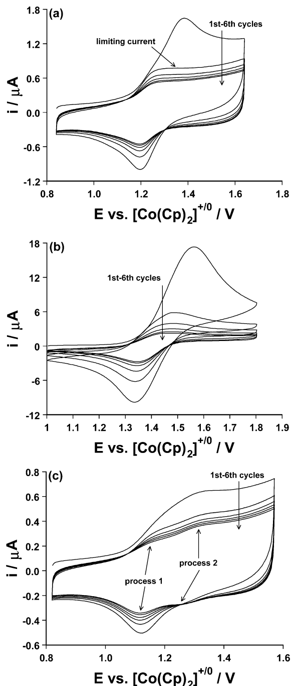
Figure 5. Cyclic voltammograms obtained at a scan rate of 0.2 \text{ V s}^{-1} when microparticles of (a) \text{Me}_2\text{DPFc} , (b) \text{Br}_2\text{DPFc} , and (c) \text{Me}_{10}\text{DPFc} adhered to a 1.5 mm diameter GC electrode are in contact with DCM (0.1 M \text{Bu}_4\text{NPF}_6 ). \text{Me}_{10}\text{DPFc}^{+/0}(\text{DCM}) reaction, as are many of the other voltammetric characteristics associated with this solution phase process. Consequently, process 1 is assigned to the reaction scheme in eq 6. The second process is then logically assigned to a fully solid-state process (eq 7), the implication being that the very high local concentration of the dissolved \text{Me}_{10}\text{DPFc}^+ prevents complete dissolution of [\text{Me}_{10}\text{DPFc}][\text{PF}_6] , at least on the voltammetric time scale. 9b
