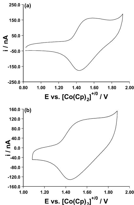
Figure 6. Cyclic voltammograms of (a) DPFc microparticles adhered to a 1 mm diameter GC electrode ( v = 0.1 \text{ V s}^{-1} ) in contact with bulk BMIM·PF 6 (scheme 2, Figure 1) and (b) as for (a) but with the microparticles being coated with a thin layer of BMIM·PF 6 prior to being placed in contact with aqueous (0.1 M KPF 6 ) electrolyte solution (scheme 3, Figure 1).
