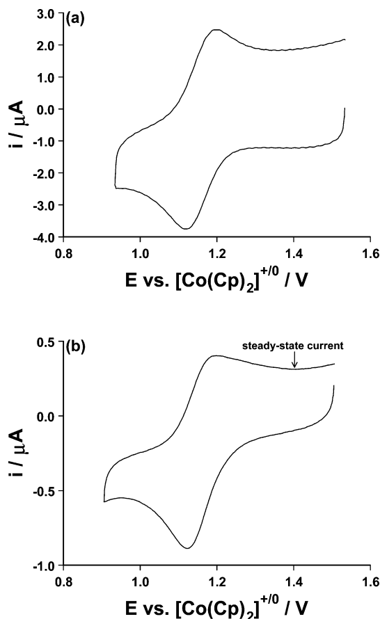
Figure 3. Cyclic voltammograms of 0.25 mM \text{Me}_{10}\text{DPFC}^+ dissolved in DCM (0.1 M \text{Bu}_4\text{NPF}_6 ) at a 1.5 mm diameter GC electrode ( v = 1 (a) and 0.1 (b) \text{V s}^{-1} ).
