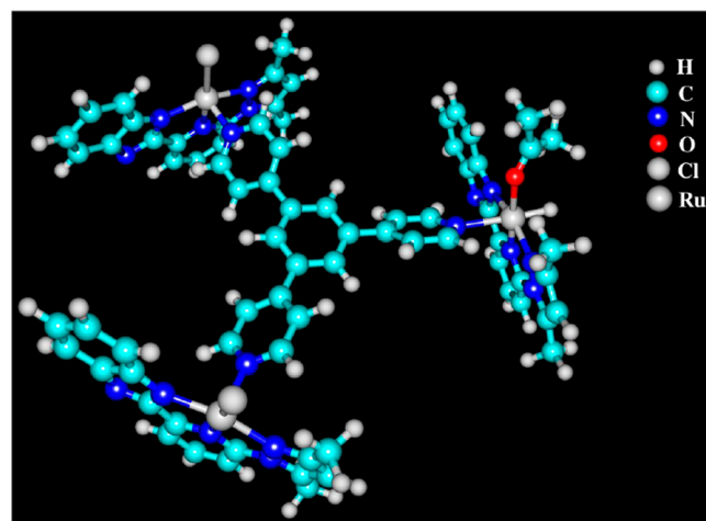
Figure 5. Optimized structure of complex 3'' .
