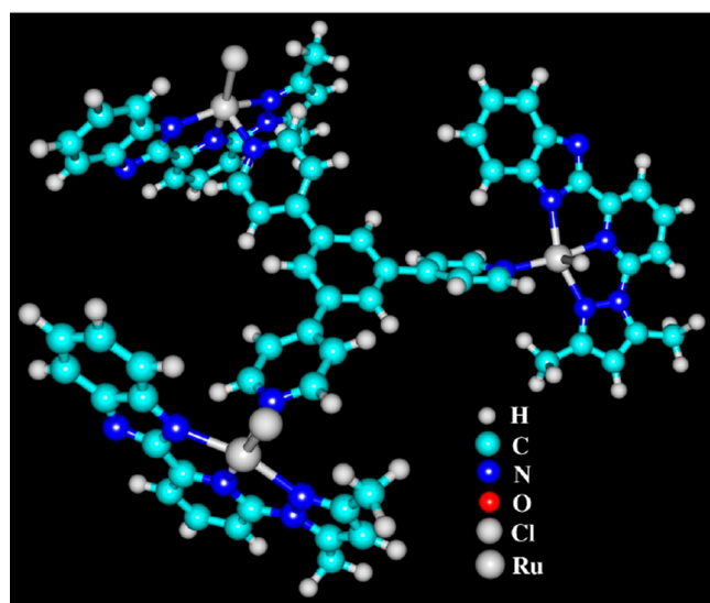
Figure 4. Optimized structure of complex 3' .
