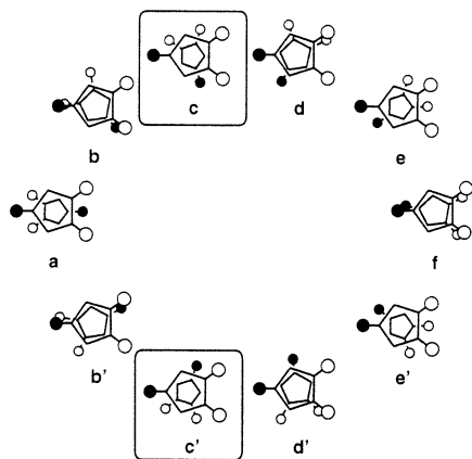
Fig. 4. Conformational analysis of 6 . Boxed diagrams correspond to the crystal structure. Filled circle = tert -butyl; open circle = \text{C}_6\text{F}_5 (Fig. 3).
