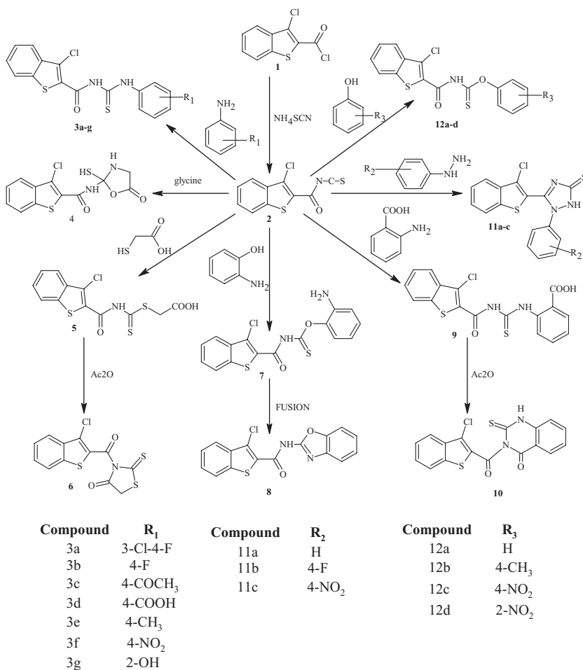
Scheme 1 General synthetic procedure for 3-chlorobenzothiophene substituted thioureas 3a-g , oxazole 4 , thiazolidinone 6 , benzoxazole 8 , quinoxaline 10 , triazoles 11a-d , and carbamothioates 12a-d .
