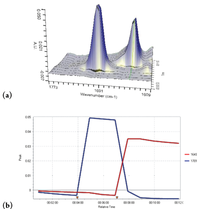
Figure 3. Investigation of the lithiation of rac -5 using n -BuLi in THF at 0 °C by in situ IR spectroscopy. (a) 3D plot showing changes in the absorption spectrum with time. (b) 2D plot showing the time evolution of the rac -5 peak at 1701 cm -1 (blue) and the lithiated intermediate 12 peak at 1643 cm -1 (red). The first and second red triangles indicate the additions of rac -5 and n -BuLi, respectively.
