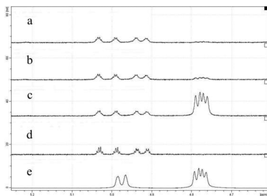
Figure 4. Investigation of the lithiation of rac -5 using n -BuLi in THF- d 8 by 1 H NMR spectroscopy: (e) rac -5 at -72 °C; (d) n -BuLi in THF- d 8 at -63 °C; (c) rac -5 + n -BuLi at -72 °C; (b) rac -5 + n -BuLi after warming to -58 °C; (a) rac -5 + n -BuLi at -58 °C after 20 min.
