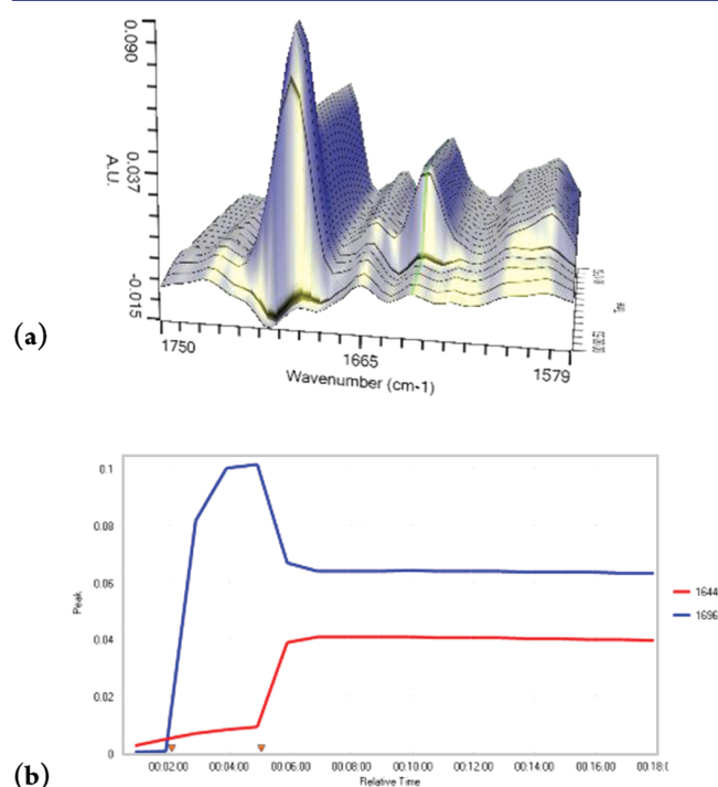
Figure 2. Investigation of the lithiation of rac-5 using n -BuLi in THF at -78^\circ\text{C} by in situ IR spectroscopy. (a) 3D plot showing changes in the absorption spectrum with time. (b) 2D plot showing the time evolution of the rac-5 peak at 1696\text{ cm}^{-1} (blue) and the lithiated intermediate 12 peak at 1644\text{ cm}^{-1} (red). The first and second red triangles indicate the additions of rac-5 and n -BuLi, respectively.
