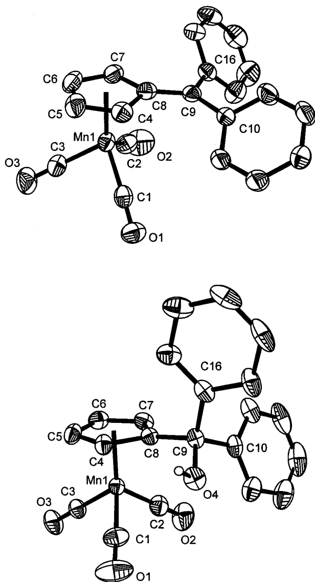
Figure 1. ORTEP drawing of 2b (top) and 7 . The core atoms are labeled. Ellipsoids are at the 50% probability level. The hydrogen atoms except for H4 have been omitted for the sake of clarity.
