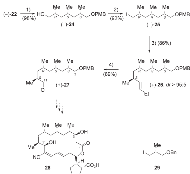
Scheme 5. Formal total synthesis (C3–C11 fragment) of borrelidin 28 via iterative directed allylic substitution. 1) \text{O}_3 , \text{NaBH}_4 , ( \rightarrow 24 ); 2) \text{PPh}_3\text{I}_2 , Im; 3) 2 equiv t\text{BuLi} , \text{MgBr}_2\cdot\text{OEt}_2 , then ( S )-( - )- 8 , \text{CuBr}\cdot\text{SMe}_2 , \text{Et}_2\text{O} ; 4) \text{O}_3 , \text{PPh}_3 .
