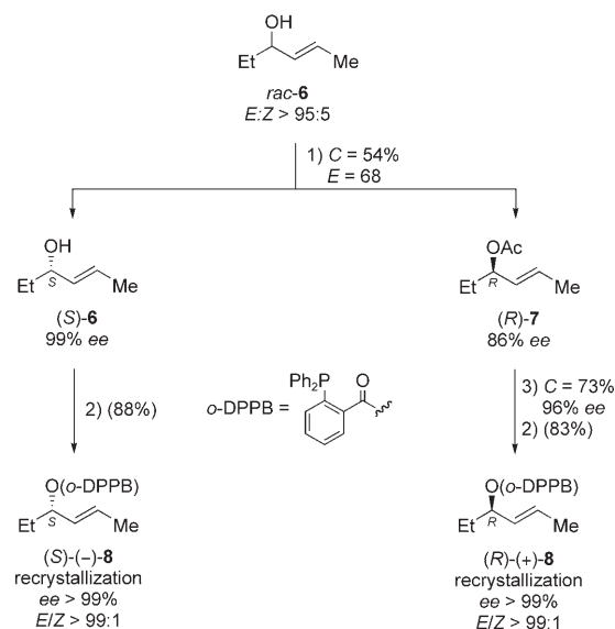
Scheme 2. Preparation of enantiomerically pure o -DPPB allylic esters 8 . 1) Novozym 435, vinylacetate, n -pentane, 30°C; 2) o -DPPBA, DCC, DMAP, CH 2 Cl 2 ; 3) Novozym 435, pH 7 buffer, 5°C; DCC: dicyclohexylcarbodiimide.
