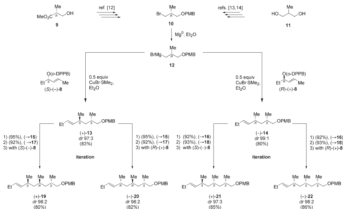
Scheme 3. Enantioselective construction of di- and trideoxypropionate building blocks based on iterative o -DPPB-directed copper-mediated allylic substitution. 1) O 3 , NaBH 4 ; 2) PPh 3 I 2 , Im; 3) 2 equiv t BuLi, MgBr 2 ·OEt 2 , then (S)-(-)-8, CuBr·SMe 2 , Et 2 O.
