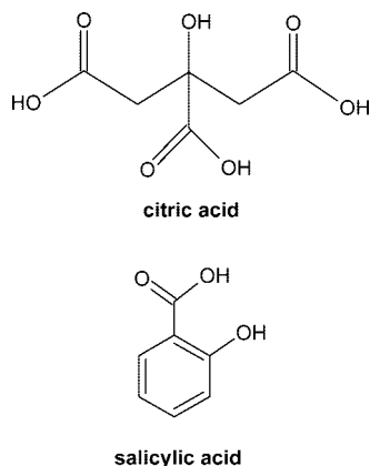
Figure 1. Structures of citric acid ( \text{H}_3\text{cit} ) and salicylic acid ( \text{H}_2\text{sal} ).
