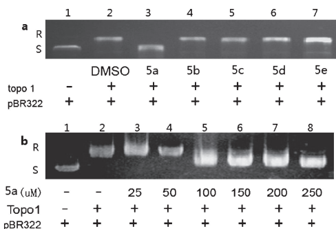
Figure 2. Effect of the compounds on the relaxation of plasmid DNA by human topoisomerase 1. (a) Lane 1, DNA pBR322; Lane 2, topo 1 + DNA pBR322 + DMSO; Lanes 3–7, DNA pBR322 relaxation by topo 1 and 5a , 5b , 5c , 5d , and 5e at concentrations of 200 \mu M, respectively. (b) Lane 1, DNA pBR322; Lane 2, topo 1 + DNA pBR322; Lanes 3–8, DNA pBR322 relaxation by topo 1 and 5a at concentrations of 25, 50, 100, 150, 200, and 250 \mu M, respectively.
