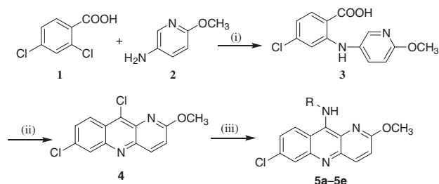
Scheme 1. Synthesis of azaacridine derivatives 5 . Reagents and conditions: (i) K 2 CO 3 , Cu, DMF, 130 °C; (ii) POCl 3 , 140 °C; (iii) various anilines, CHCl 3 , EtOH, concd HCl.
