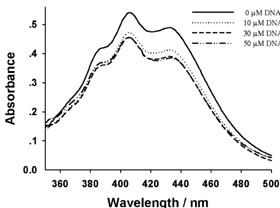
Figure 1. UV-visible absorption spectra of azaacridine analogue 5a (50 \mu M) in the absence (solid line) or presence (dashed line) of increasing amounts of ct DNA.
