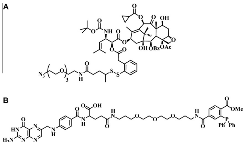
Scheme 1. Structures of az-SBT1214 and phosphine-folate used to chemoselectively modify O-GlcNAz and HPG labeled Ad-Luc.
