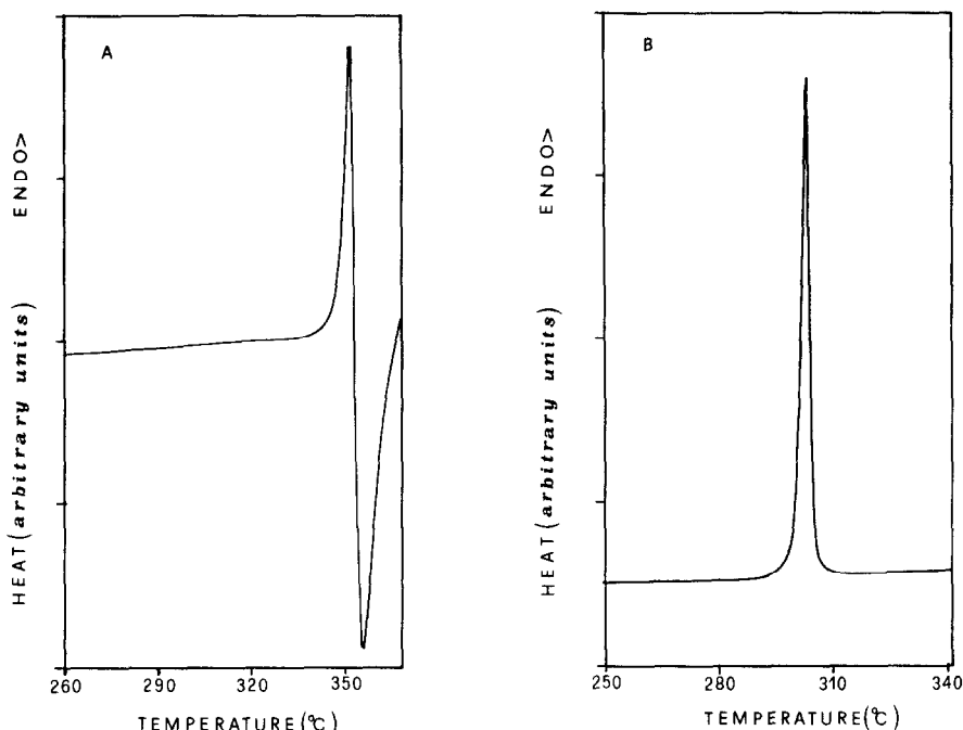
Fig. 4. DSC profiles of 1d (A) and 1f (B) (40 °C/min, N 2 ).
