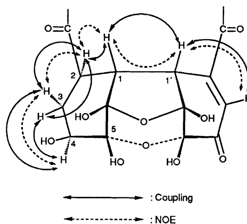
Figure 1. ^1\text{H} – ^1\text{H} and NOE correlations in (9).
