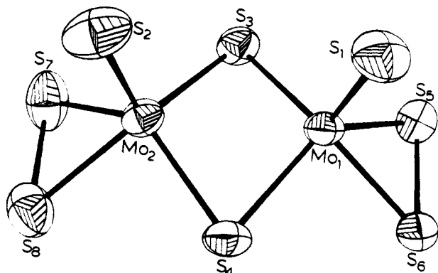
Figure 1. The structure of \text{Mo}_2\text{S}_8^{2-} as determined in its (\text{C}_6\text{H}_5)_4\text{P}^+ salt. Bond distances and angles in the anion are: \text{Mo}_1\text{--Mo}_2 = 2.821 (1), \text{Mo}_2\text{--S}_2 = 2.108 (1), \text{Mo}_1\text{--S}_1 = 2.128 (1), \text{S}_5\text{--S}_6 = 2.051 (2), \text{S}_7\text{--S}_8 = 2.072 (3), \text{Mo}_2\text{--S}_7 = 2.391 (1), \text{Mo}_2\text{--S}_8 = 2.405 (2), \text{Mo}_1\text{--S}_5 = 2.403 (1), \text{Mo}_1\text{--S}_6 = 2.375 (2), \text{Mo}_2\text{--S}_3 = 2.314 (1), \text{Mo}_2\text{--S}_4 = 2.313 (1), \text{Mo}_1\text{--S}_3 = 2.306 (1), \text{Mo}_1\text{--S}_4 = 2.308 (2) Å; \text{S}_4\text{--Mo}_2\text{S}_3 101.0 (1)°, \text{S}_4\text{--Mo}_1\text{--S}_3 101.4 °, \text{Mo}_1\text{--S}_3\text{--Mo}_2 75.3 (1)°, \text{Mo}_1\text{--S}_4\text{--Mo}_2 75.2 (1)°.
