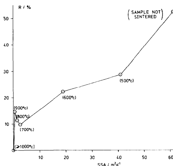
Fig. 4. Relationship between SSA of zinc sulphide and extent of its reaction ( R ) with aqueous copper(II) sulphate. R is defined by: R = [(C - T)/C] \times 100\% . C and T are the concentrations of aqueous copper(II) in control and test solutions respectively.
