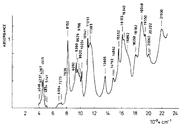
Fig. 1. Absorption spectrum.
