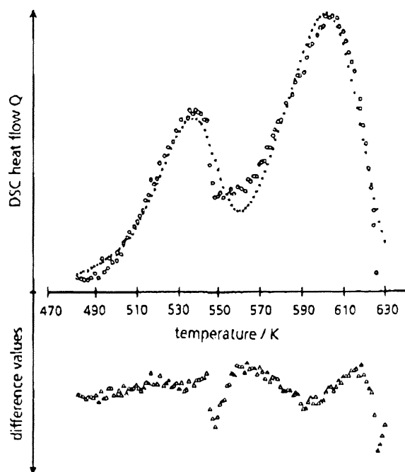
Fig. 3. Plots of the deconvoluted DSC curve (○), the best fit curve (■) of the two-step reaction model and the difference (Δ) of the two curves. Original DSC data recorded at 2 K/min and 0.15 g/cm 3 loading density.
