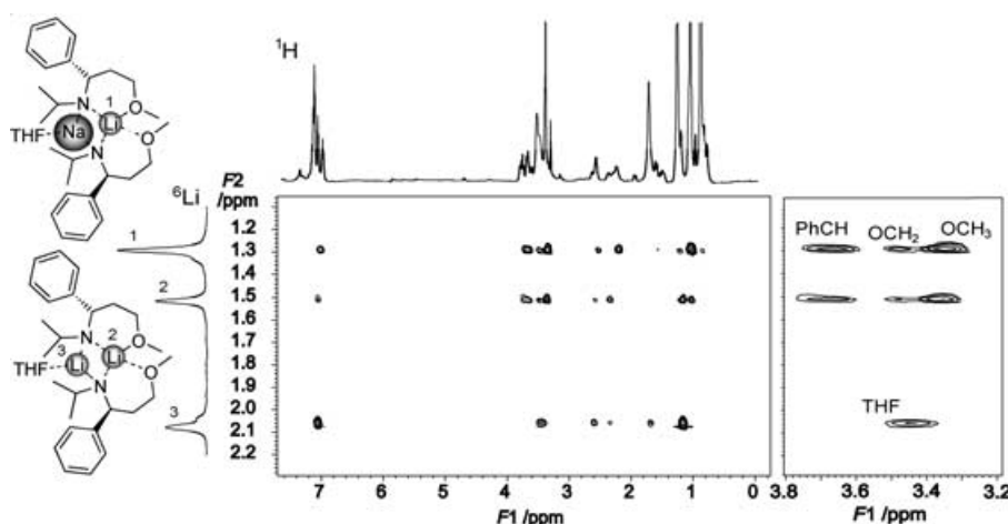
Figure 3. ^6\text{Li}, ^1\text{H} HOESY spectrum of 1 (0.18 mmol), n BuNa (0.07 mmol), n BuLi (0.11 mmol), and THF (0.11 mmol) in [\text{D}_{10}]\text{Et}_2\text{O} (0.6 mL) at -88^\circ\text{C} , with scale expansion of the ^1\text{H} spectral region ( \delta = 3.2\text{--}3.8 ppm) shown on the right.
