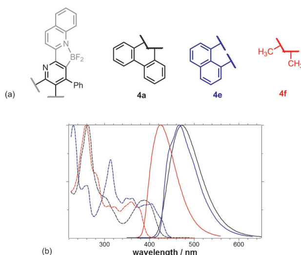
Figure 6. Normalized absorption (left) and emission spectra (right) of compounds 4a , 4e and 4f in \text{CH}_2\text{Cl}_2 . The color of the depicted subunits in (a) indicates the color of the respective spectra in (b).
