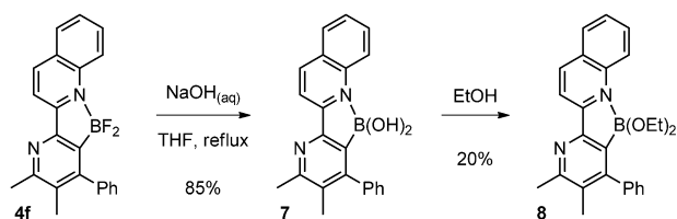
Scheme 3. Synthesis of 7 and 8 .
