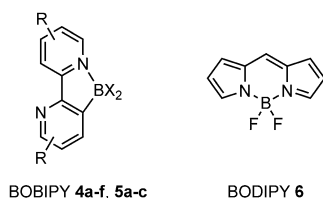
Figure 2. General structure of BOBIPYs (4a–f, 5a–c) and BODIPY 6 used for comparison of optical properties.
