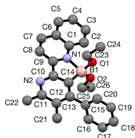
Figure 8. ORTEP of BOBIPY 8 . Hydrogen atoms are omitted for clarity. Selected bond lengths [Å] and angles [°]: N1-B1 1.762(2), C14-B1 1.628(3), O1-B1 1.425(3), O2-B1 1.420(2); N1-C9-C10-C14 2.95(2), C8-C9-C10-N2 2.64(3).
