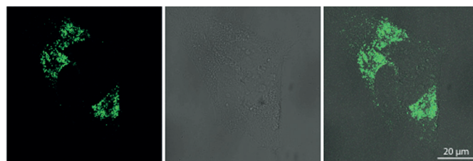
Figure 10. Fluorescent confocal microscopy of 10 in HeLa cells. Left: Emission at 458 nm, Excitation: at 458 nm; Middle: Brightfield; Right: Merge. For further conditions see SI.
