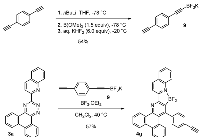
Scheme 4. Synthesis of 4g .
