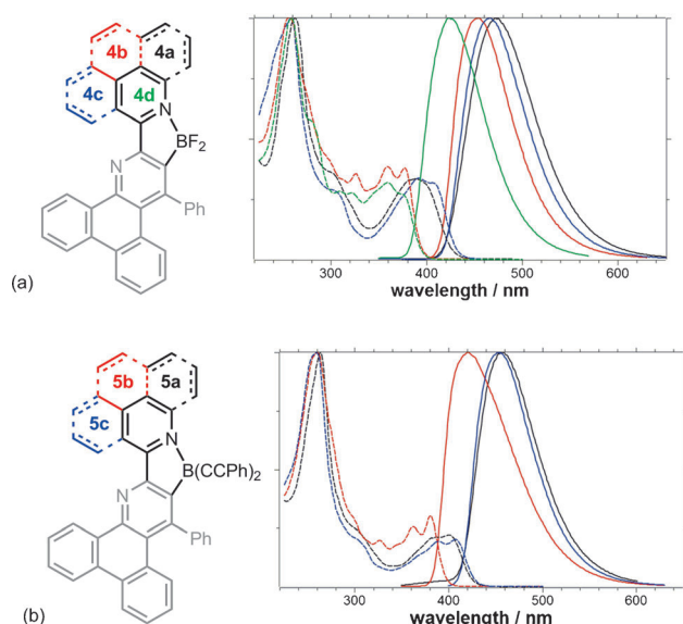
Figure 5. Normalized absorption (left) and emission spectra (right) of compounds 4a–d (a) and 5a–c (b) in \text{CH}_2\text{Cl}_2 . The color of the ring systems indicates the color of the respective spectra in (a) and (b).
