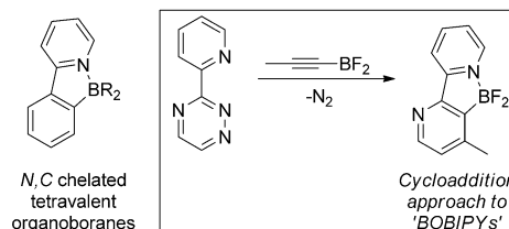
Scheme 1. Directed cycloaddition approach to fluorescent BOBIPYs.
