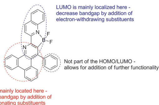
Figure 9. Modification of the fluorophore 4a allows for further color-tuning or the addition of more functionalities.
