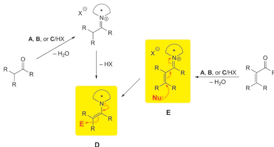
Scheme 2. Reactive Intermediates D and E Formed from the Pyrrolidine and Imidazolidinone Catalysts A–C, and Carbonyl Compounds. The enamine D reacts with electrophiles ( d^2 -reactivity [18]) and the enoyl-iminium ion E with nucleophiles ( a^3 -reactivity). The conjugate, Michael -type addition to E produces an enamine of type D , which, in turn, can couple intra - or intermolecularly with an electrophilic center. Vinylogous cases, in which a dienamine exerts d^4 -reactivity, or a dienoyl-iminium ion a^5 -reactivity, are also known [1].
