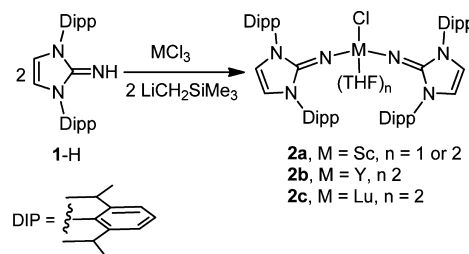
Scheme 2. Syntheses of the Bis(imidazolin-2-iminato) Complexes [(\text{Im}^{\text{Dipp}}\text{N})_2\text{MCl}(\text{THF})_n] ( 2a–2c )
