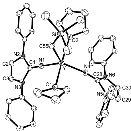
Figure 6. ORTEP diagram of 4b in 4b - n -pentane with thermal displacement parameters drawn at 50% probability. The isopropyl groups have been omitted for clarity.
