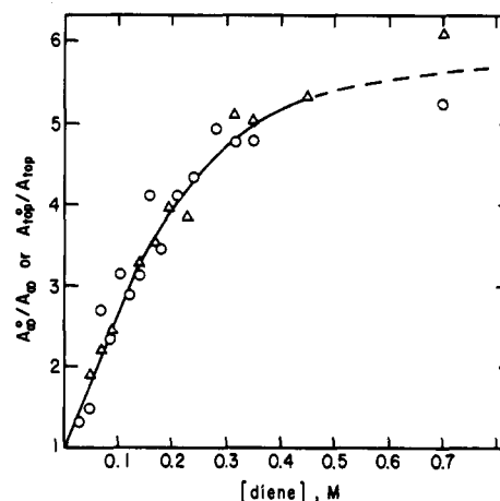
Figure 5. Quenching data according to eq 7 (O) for 3 and similar plot monitoring the "top" absorbances at 400 nm in the absence of PQ^{2+} ( \Delta ).
