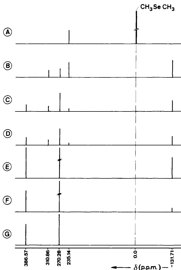
Figure 2. 77 Se NMR spectra of \alpha -(methylseleno)- p -nitrostyrene ( 5 \times 10^{-4} mol) in methanol (A) without acid and (B–G) in the presence of 2 \times 10^{-3} mol of \text{H}_2\text{SO}_4 after 45, 70, 120, 165, 270, and 370 min, respectively. Spectra A–D were obtained from 300 scans and E–G resulted from 2000 scans.
