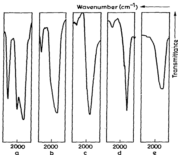
Fig. 4. a) The IR spectrum of the reaction mixture of benzyl alcohol and \text{RuCl}_2(\text{PPh}_3)_3 in dibenzyl ether at 190°C. b) The IR spectrum of the reaction mixture after 0.5 h. c) The IR spectrum (in Nujol) of the residue from the reaction mixture. d) The IR spectrum of the product isolated from the reaction mixture. e) The IR spectrum of \text{RuCl}_2(\text{PPh}_3)_3 , benzyl alcohol, and benzylideneacetone after 50 min at 200°C.
