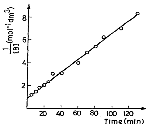
Fig. 1. Plot of the reciprocal concentration of benzylideneacetone [\text{B}] (benzyl alcohol) vs. time. 3.46 \times 10^{-3} \text{ M} \text{RuCl}_2(\text{PPh}_3)_3 , 1.1 \text{M} benzylideneacetone, and 1.1 \text{M} benzyl alcohol in dibenzyl ether; reaction temperature 190°C, total volume: 4 ml.
